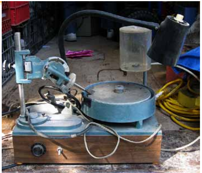
Graves faceting machine
